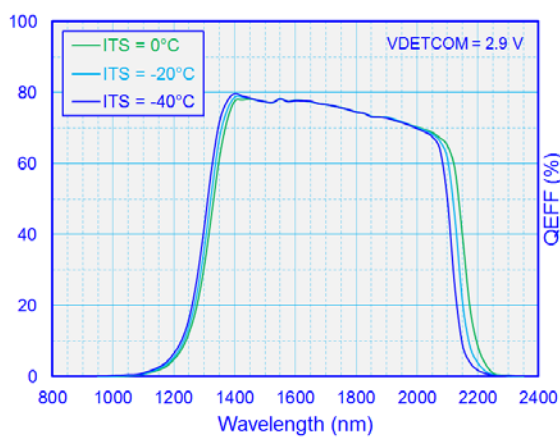
QEFF Spectrum
