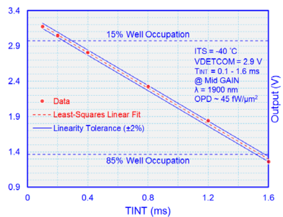
Output Linearity
